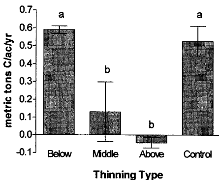
Figure 2. Average annual change in carbon stocks for the period 1975–2000, in metric tons of carbon per acre per year. Pools included are live biomass, deadwood, logging residue, and products. Error bars are standard error of the mean. Bars with the same lower case letter above the bar are not significantly different.
