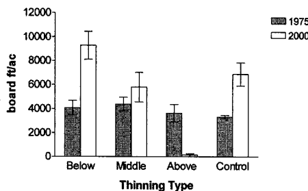
Figure 3. Merchantable volume, in bd ft per acre, before treatment and in 2000 after two thinnings. Error bars are standard error of the mean.
