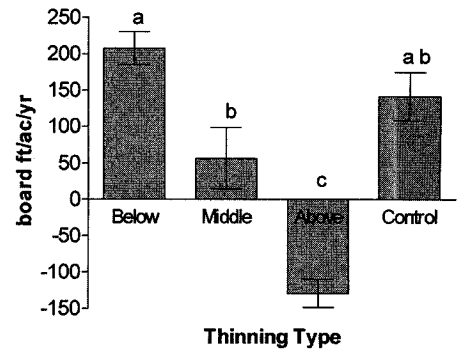
Figure 4. Average annual change in merchantable volume for the period 1975–2000, in bd ft per acre per year. Error bars are standard error of the mean. Bars with the same lower case letter above the bar are not significantly different.
