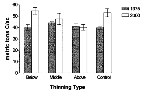
Figure 1. Carbon stocks, in metric tons per acre, before treatment and in 2000 after two thinnings. Carbon pools include live biomass (including coarse roots) for the pre-treatment case, and live biomass, deadwood, logging residue, and products for the post-treatment case. Error bars are standard error of the mean.
